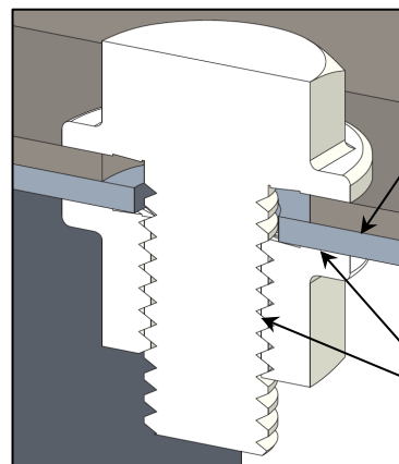
Image 21: Friction within the solar PV bolted joint prevents joint slip and the resulting self-loosening in a properly designed and assembled bolted joint.
