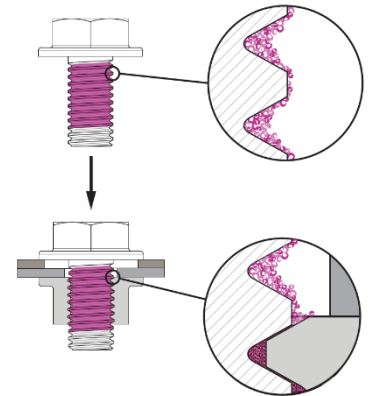
Image 27: Pre-applied thread locker is activated upon assembly of the bolted joint.
