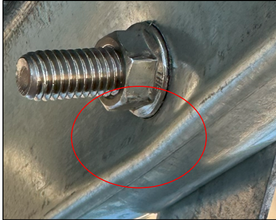
Image 9: Example of a ‘hat’ section yielding due to the pretension of in bolt.
