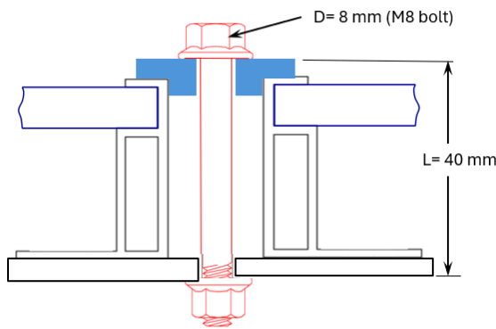
Image 17: Typical PV Module Top-Down Clamp Bolted Joint
