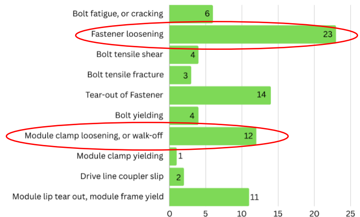
Figure 1: Summary of Failure Mechanisms Reported in SETO Solar PV bolted joint Failure Survey
