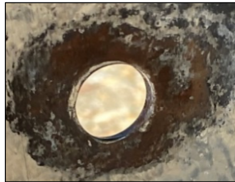
Image 13: Example of fretting wear of G90 purlin at the joint interface due to repeated joint slip.
